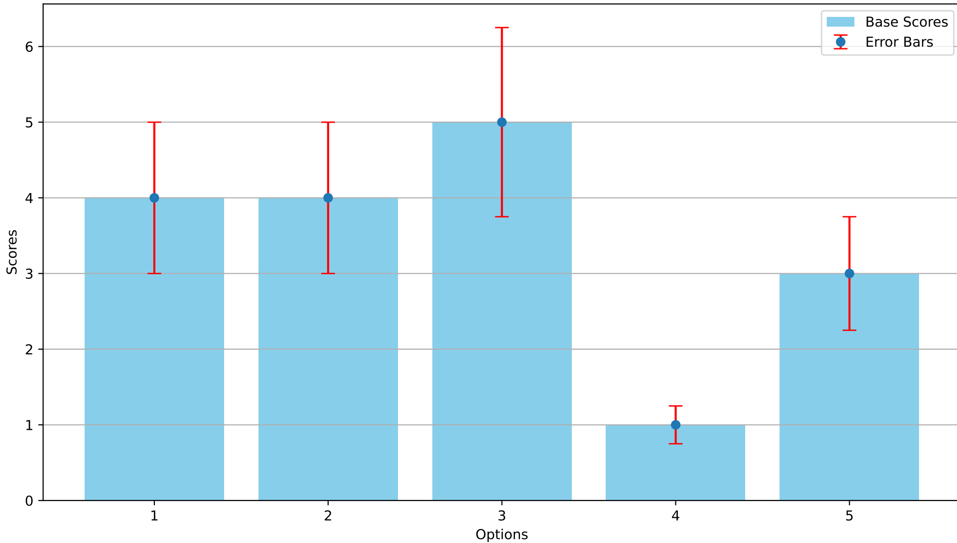
Combined Result Sensitivity Analysis for Payload Capacity
